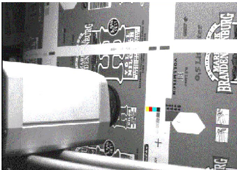
Figure 1. Online spectral imaging in printing control
